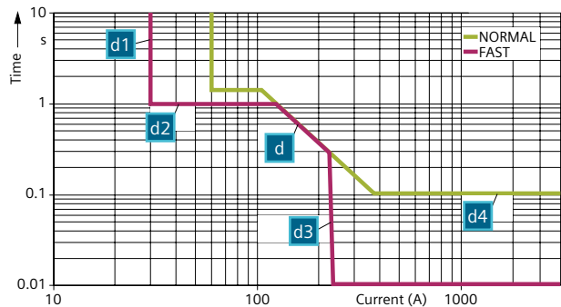
Fuse replacement protection – time-current curve
