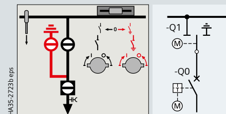
馈线分闸
