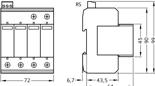
3+1 5SD74T2
