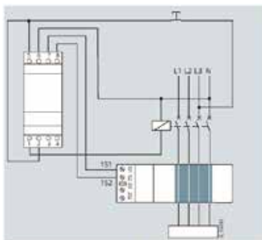
剩余电流监测装置, SSV8000-4KK, 短路脱扣器 (ST)
