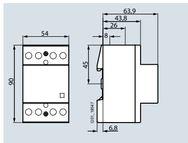
5TT5041-0 5TT5041-2
