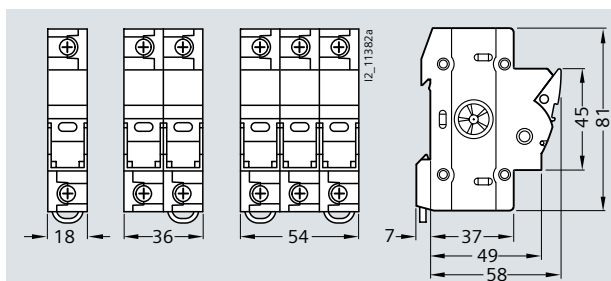
3NC1 091/3NC1 092/3NC1 093
