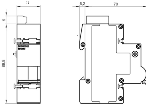
5ST3053
