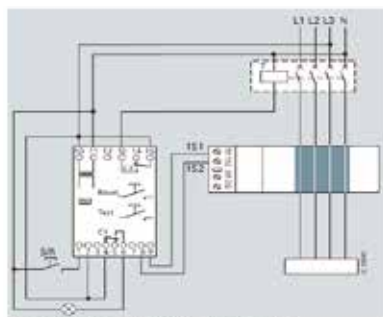
剩余电流监测装置, SSV8001-4KK, 短路脱扣器 (ST)
