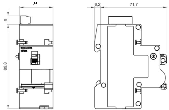
5ST3054
