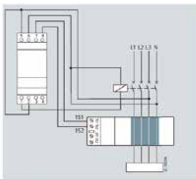
剩余电流监测装置, SSV8000-6KK, 短路脱扣器 (ST), 欠电压
