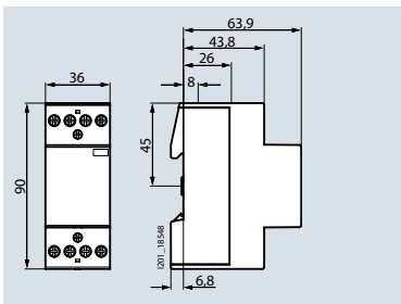
5TT5032-0 5TT5032-2
